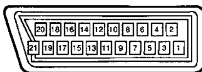
21-PIN TERMINAL
