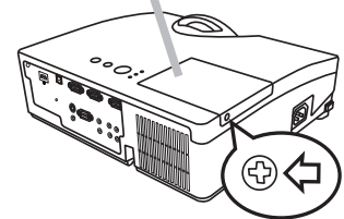
lamp cover
