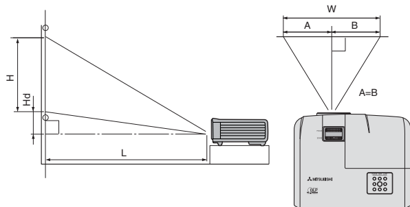
L: Between the screen and the front edge of the projector H: Height of the projected image
