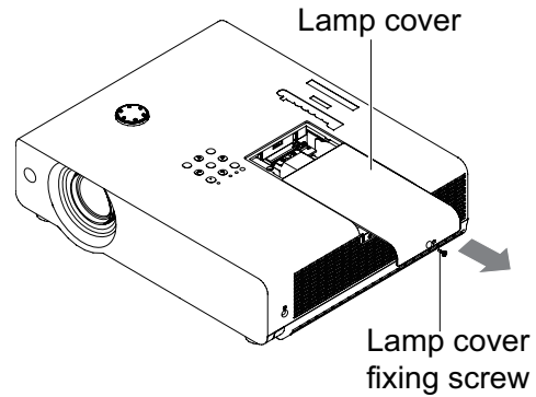
Lamp unit fixing screws
