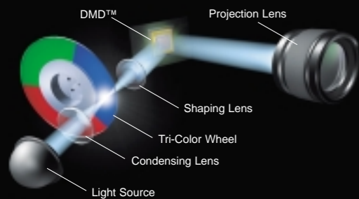
The DPX-1 Optical System
