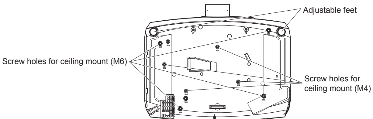
The positions of screw holes for ceiling mount and adjustable feet
