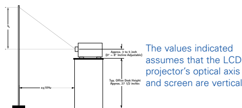
a: LCD projector to screen distance b: Distance from lens center to screen top/bottom
