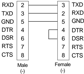
<Fig.1, RS-232 Interface Cable>
