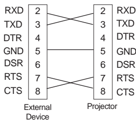
<Fig.1, RS-232 Interface Cable>
