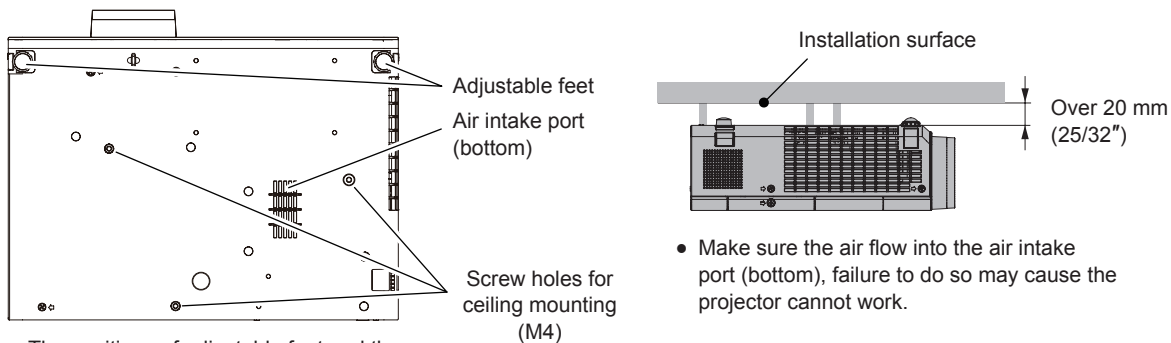
The positions of adjustable feet and the screw holes for ceiling mounting
