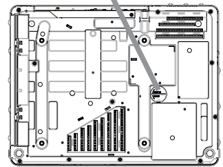
Battery Cover
