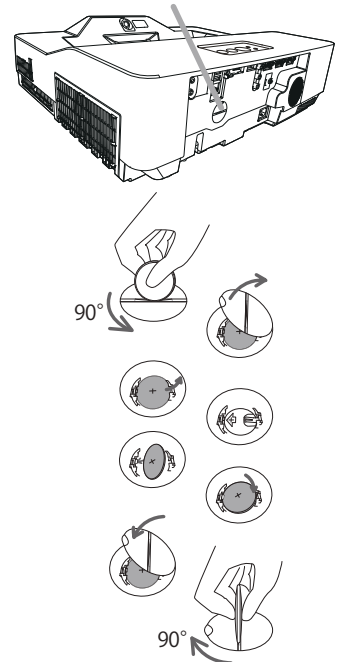
Battery Cover
