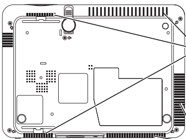
Exhaust Vent (Hot air exhaust)
