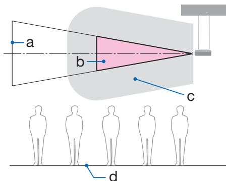
a: Screen / b: Hazard zone / c: Precautionary zone / d: floor
